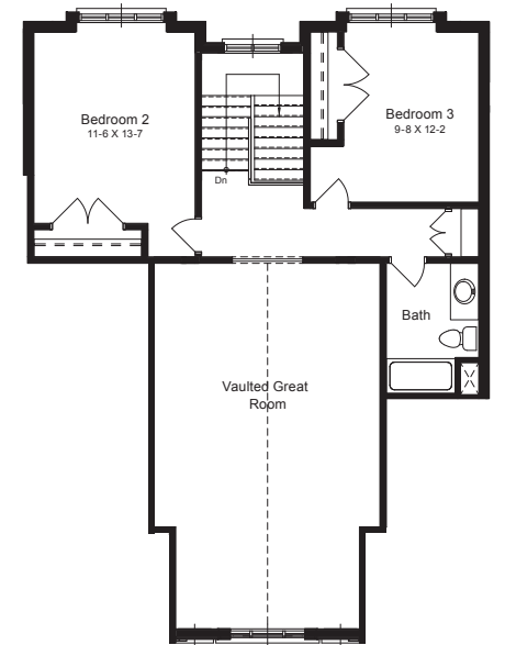
SECOND LEVEL
